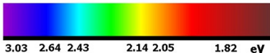
Figure 4. Energy of separated photons of coronal glow
