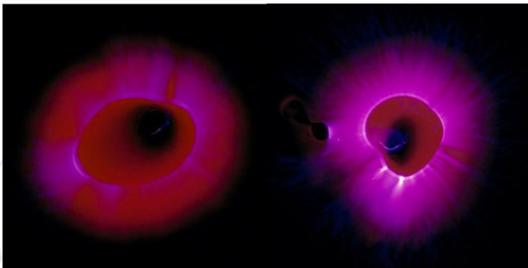
Figure 3. Color coronal images of the control sample in right and the sample Desert Greening Orgone device in left.
